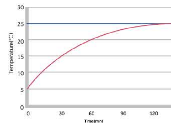
HYC-390 Warm-up test at 25°C ambient
