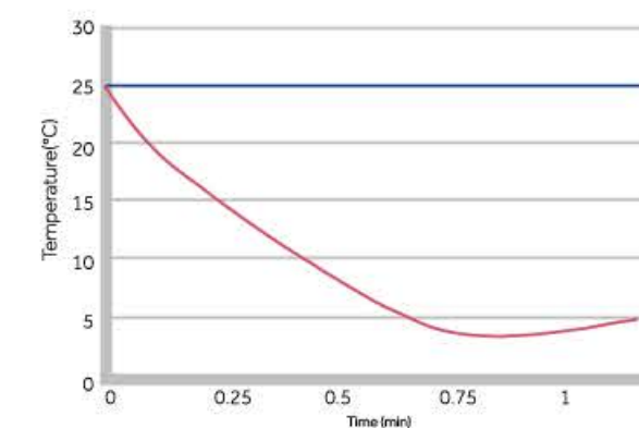
HYC-390 Pull down test at 25°C ambient
